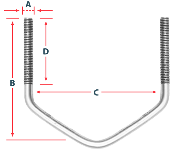
A = Diameter B = Inside Length C = Inside Width D = Thread Length
