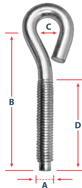
A = Diameter B = Length Centre Eye C = Eye Diameter D = Thread Length
