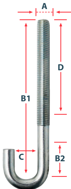
A = Diameter B1 = Inside Length 1 B2 = Inside Length 2 C = Inside Width D = Thread Length
